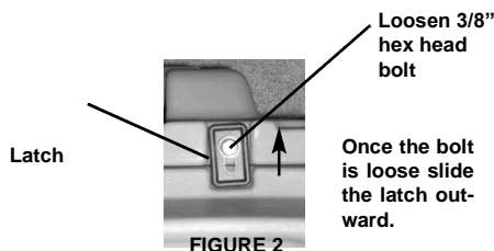
Loosening the latches
